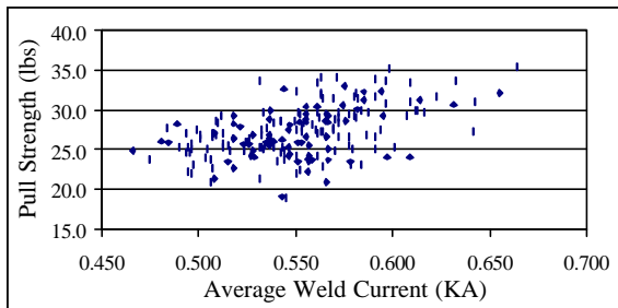
Figure 1 - Pull strength versus weld current.
