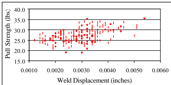
Figure 2 - Pull strength versus weld displacement.
